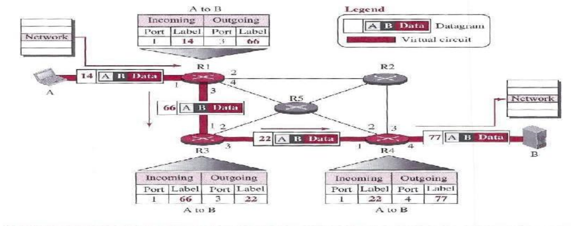
Flow of one packet in an established virtual circuit
