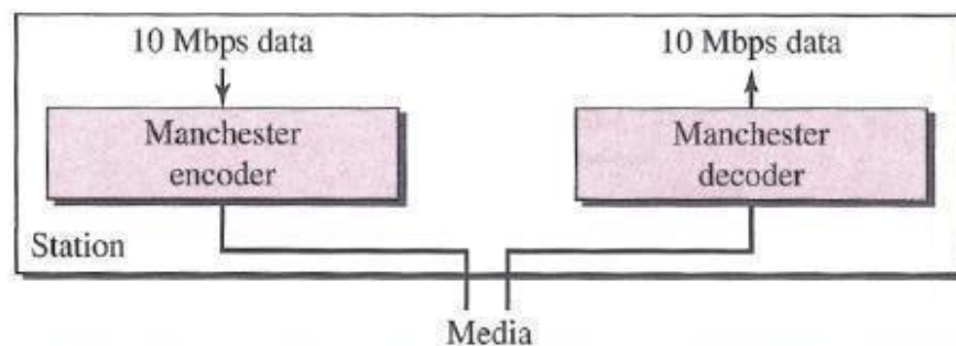
Encoding in a Standard Ethernet implementation
