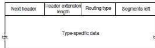
The extension header for routing
